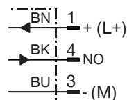
Connection diagram
