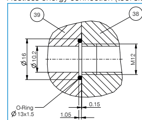
Hoseless Energy connection (robot side)
