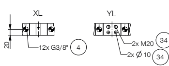
Hostless energy connection (tool side)
