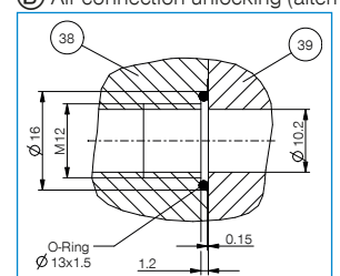
Hostless energy connection (tool side)
