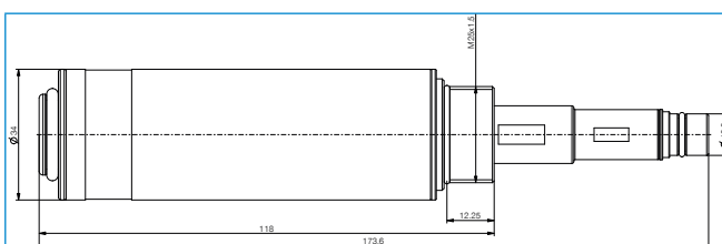
ZVC303-TS1M25
