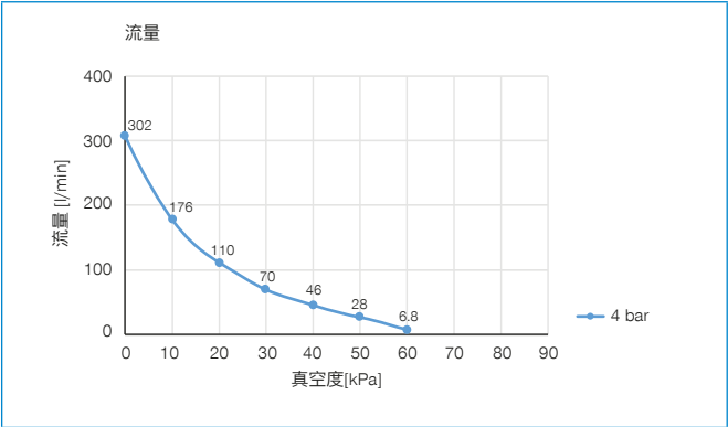
ZVCX303
