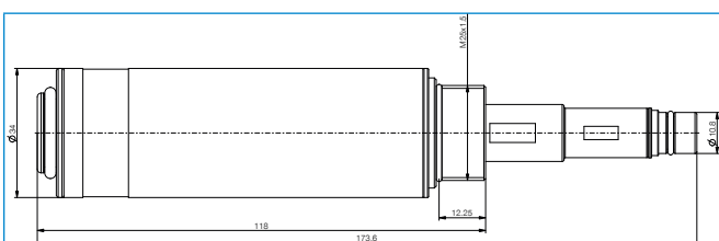
ZVC303-NRV-TS1M25
