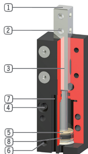
Fig. 2: VEG separator cross-section
